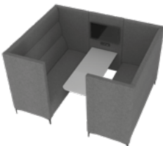
Huddle Cave Six Seater (Media) width 2270, depth 1960, height 1490, seat height 440 mm
