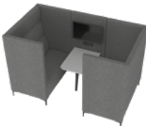
Huddle Cave Four Seater (Media) width 2270, depth 1360, height 1490, seat height 440 mm
